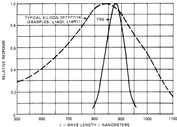
5. SPECTRAL RESPONSE
