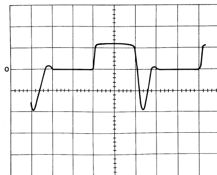
V = 50 \text{ V/DIVISION} t = 200 \text{ ns/DIVISION}
