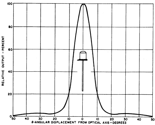
5. 1N6264 - TYPICAL RADIATION PATTERN
