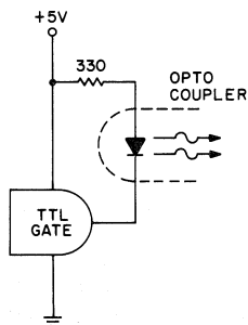
Fig. 120a - Direct connection of TTL I_o \geq 7\text{mA} .
