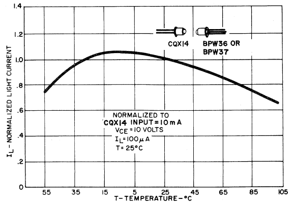
NORMALIZED LIGHT CURRENT VS TEMPERATURE Both Emitter (CQX14) and Detector (BPW36 or BPW37) at Same Temperature
