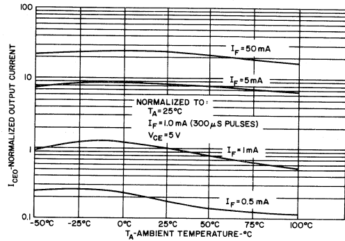
OUTPUT VS. TEMPERATURE
