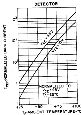
4. LEAKAGE CURRENTS VS. TEMPERATURE
