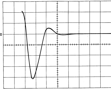
b) EXPANDED SCALE OF TURNOFF PORTION OF ABOVE WAVEFORM V = 20 \text{ V/DIVISION} t = 50 \text{ ns/DIVISION}
