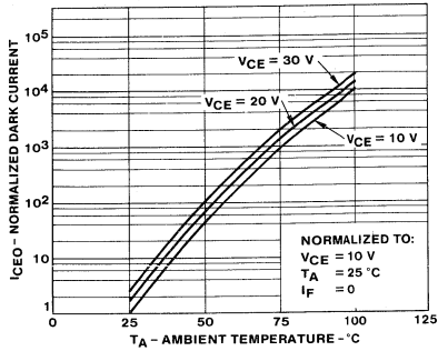
3. DARK I_{CEO} CURRENT VS TEMPERATURE
