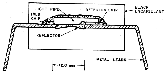
Fig. 13 - Cutaway view of General Electric H11AV; 6 pin DIP Optoisolator approved to VDE Safety Standard 0883/6.80, with testing to 0730/6.76 and 0860/11.76.
