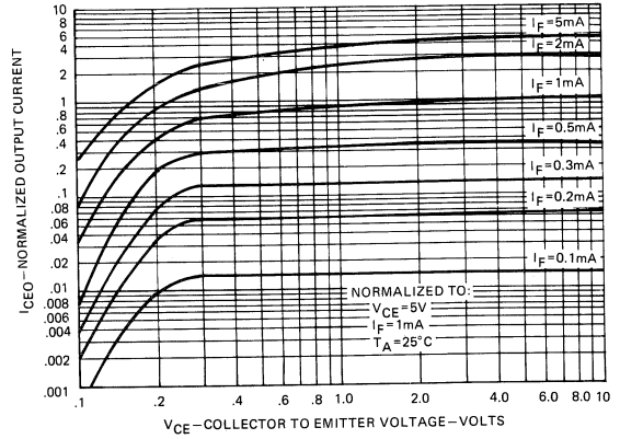
OUTPUT CURRENT VS. COLLECTOR-EMITTER VOLTAGE
