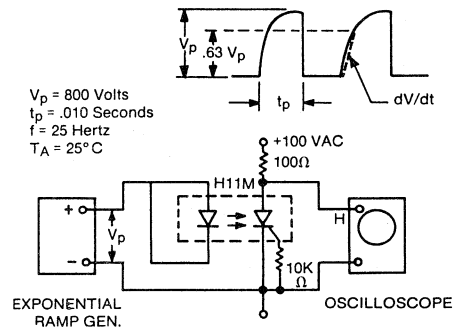
10. ISOLATION dv/dt IMMUNITY TEST CIRCUIT
