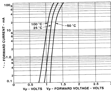
INPUT CHARACTERISTICS
