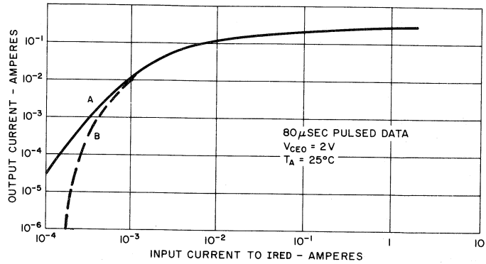
Fig. 43 - Typical photodarlington optocoupler transfer characteristics.
