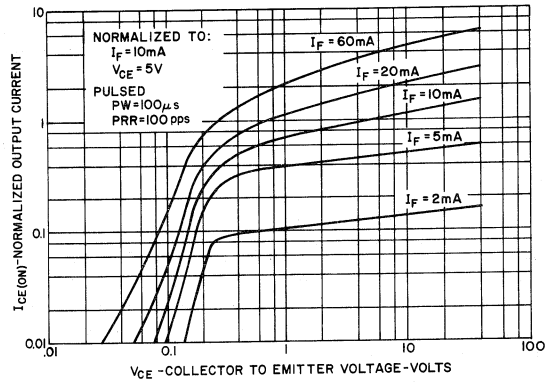
4. OUTPUT CHARACTERISTICS
