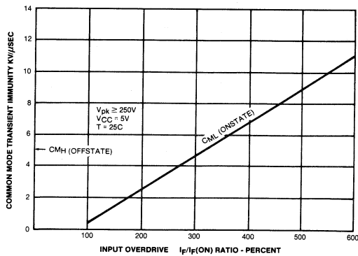
CM_L AND CM_H VS INPUT CURRENT
