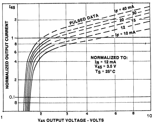
1. OUTPUT CHARACTERISTICS
