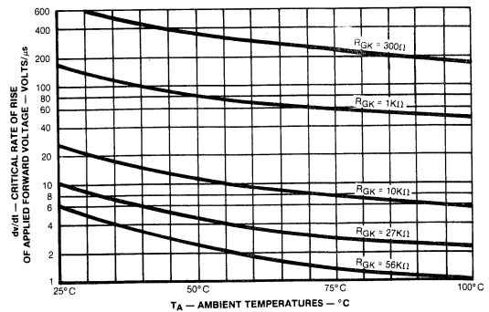
6. dv/dt VS. TEMPERATURE
