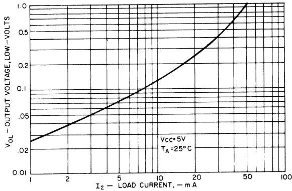
ON VOLTAGE VS. LOAD CURRENT
