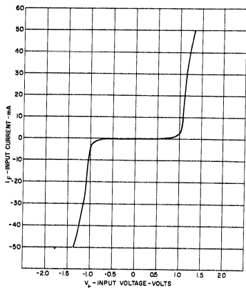
1. INPUT CHARACTERISTICS
