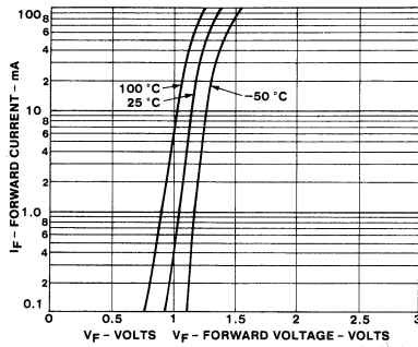
FORWARD VOLTAGE VS. FORWARD CURRENT
