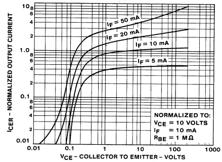
4. OUTPUT CHARACTERISTICS
