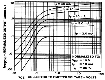
OUTPUT CHARACTERISTICS
