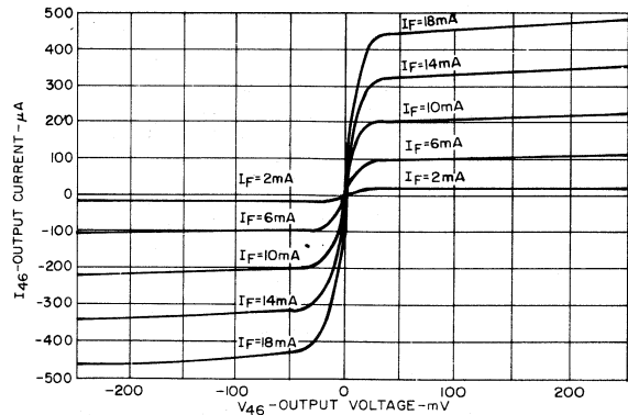
3. OUTPUT CHARACTERISTICS
