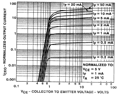
OUTPUT CHARACTERISTICS
