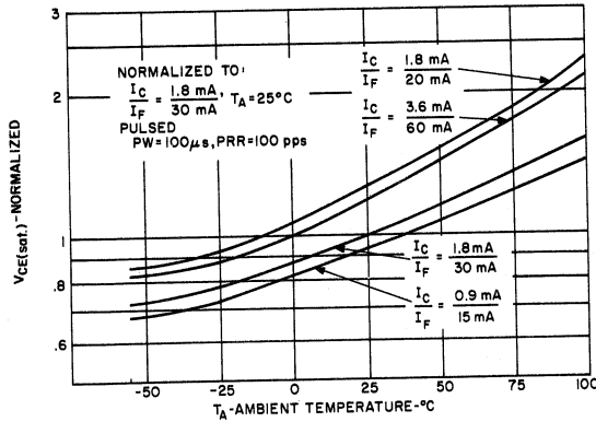
3. V_{CE}(\text{sat}) VS. TEMPERATURE
