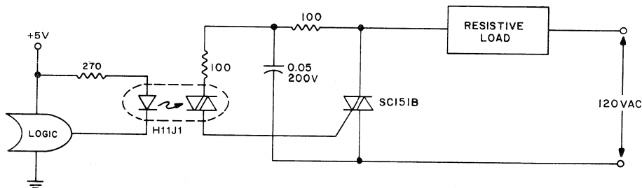
Fig. 131 - Minimum parts count isolated logic triggered triac.
