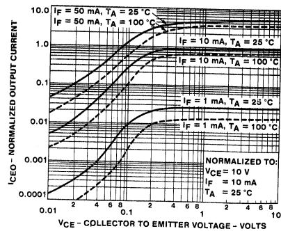
6. OUTPUT CHARACTERISTICS
