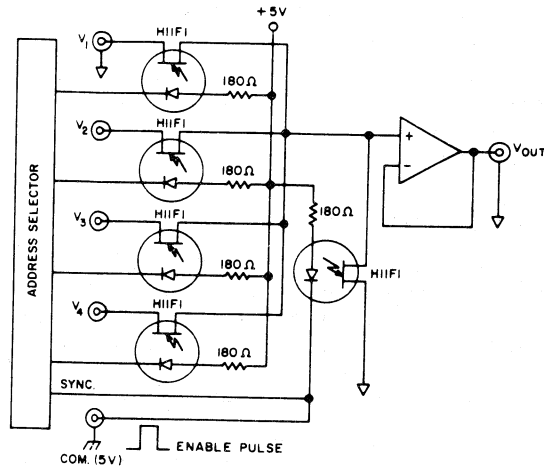
Fig. 116 - Four channel multiplexer.
