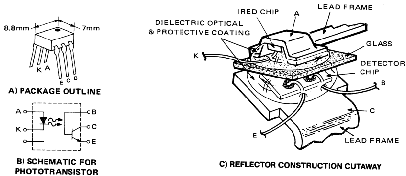
Fig. 12 - Glass dielectric construction techniques for GE 6 pin DIP.
