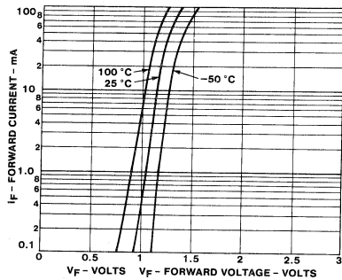
INPUT CHARACTERISTICS
