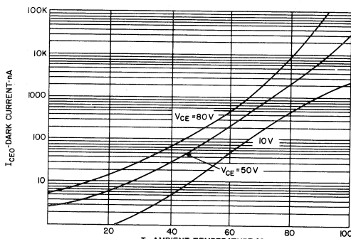
DARK CURRENT
