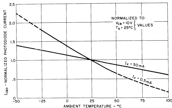
Fig. 38 - Photodiode transfer characteristics temperature variation.
