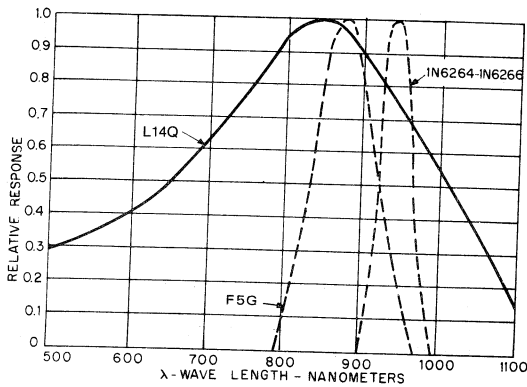
5. SPECTRAL RESPONSE
