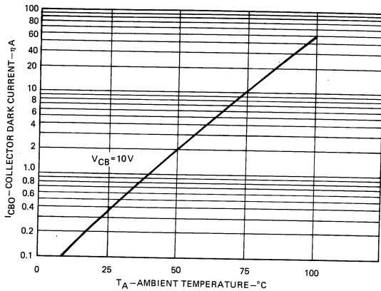
I CBO VS. TEMPERATURE
