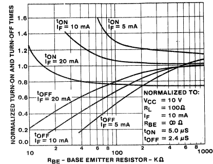
12. SWITCHING TIME VS RBE
