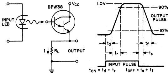
5. TEST CIRCUIT AND VOLTAGE WAVEFORMS
