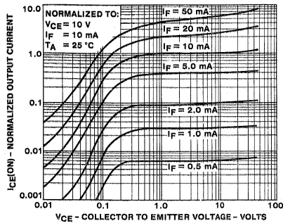
5. OUTPUT CHARACTERISTICS
