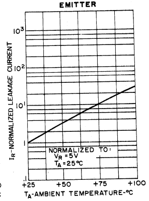
4. LEAKAGE CURRENTS VS. TEMPERATURE
