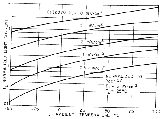
2. LIGHT CURRENT VS. AMBIENT TEMPERATURE
