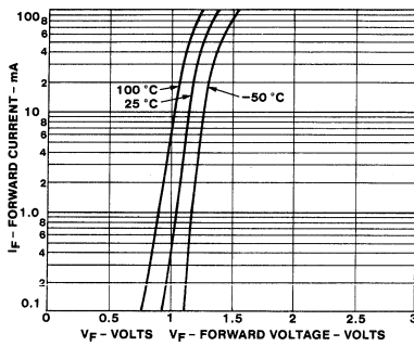
3. INPUT CHARACTERISTICS
