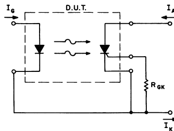
Fig. 74b - I_T tested as SCR I_{Gt} .
