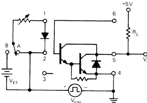
TEST CIRCUIT FOR TRANSIENT IMMUNITY AND TYPICAL WAVEFORMS
