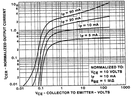
4. OUTPUT CHARACTERISTICS
