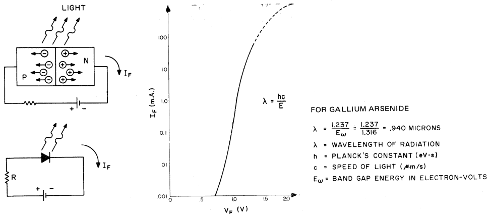
Fig. 1 - The forward biased light emitting diode pn junction.
