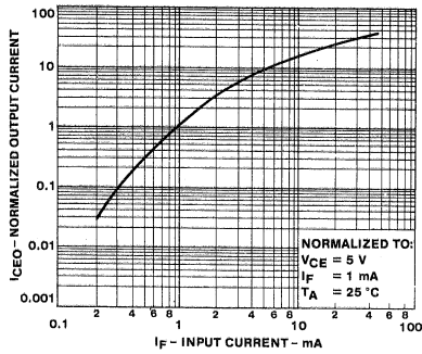
OUTPUT CURRENT VS INPUT CURRENT
