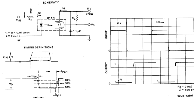
Fig. 2 - H11N schematic diagram and timing waveforms.
