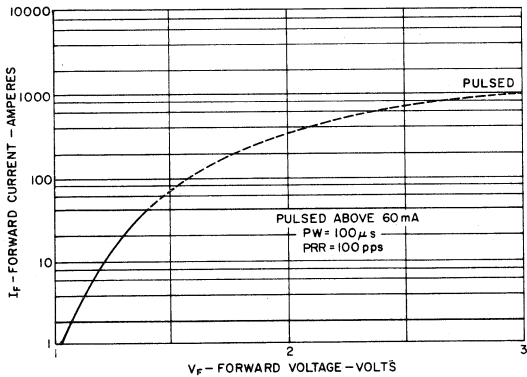
3. INPUT CHARACTERISTICS
