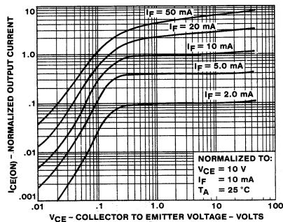
4. OUTPUT CHARACTERISTICS
