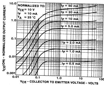
5. OUTPUT CHARACTERISTICS
