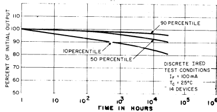
Fig. 63 - Long-term IRED life test results.
