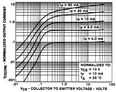
4. OUTPUT CHARACTERISTICS
