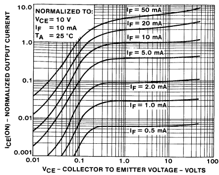
5. OUTPUT CHARACTERISTICS
