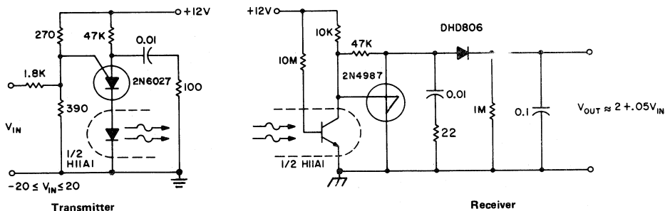
Fig. 100 - Minimum parts count linear PRM isolation circuit.
