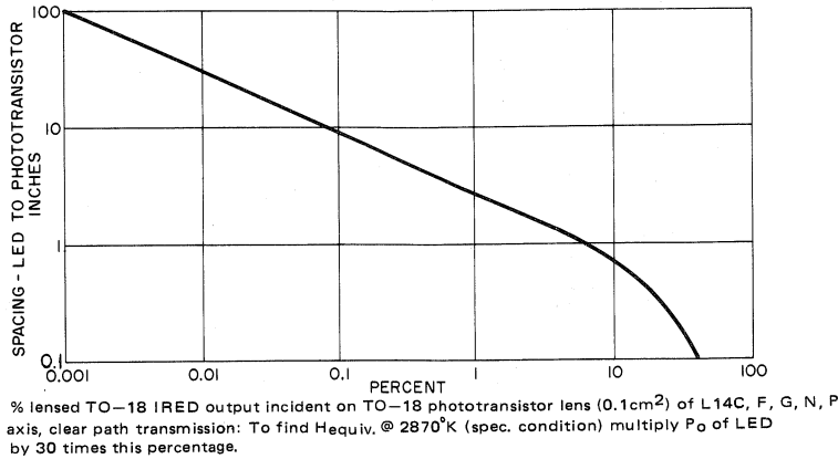
Fig. 18 - Lensed LED to phototransistor coupling chart.
