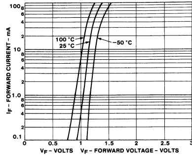
FIGURE 2. FORWARD VOLTAGE VS. FORWARD CURRENT
