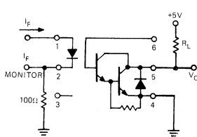
SWITCHING TEST CIRCUIT
