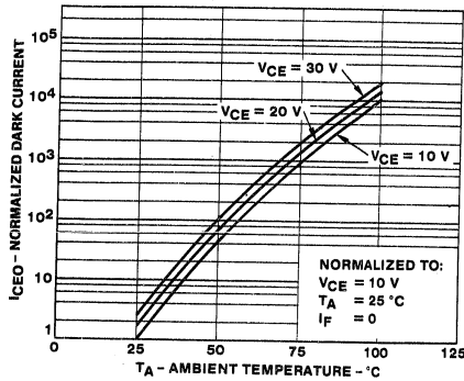
3. DARK I_{CE0} CURRENT VS. TEMPERATURE
