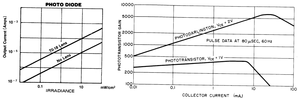
Fig. 20 - Typical photodetector current and gain.
