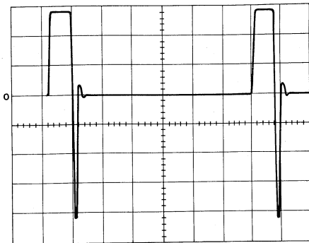
a) LOAD VOLTAGE ACROSS 45\Omega V = 20 \text{ V/DIVISION} t = 500 \text{ ns/DIVISION}
