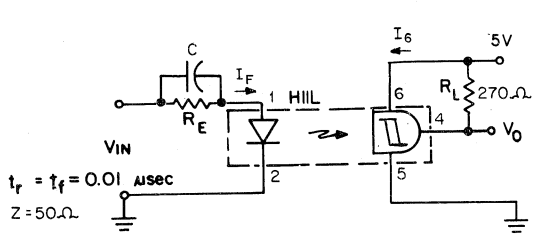
SWITCHING TEST CIRCUIT
