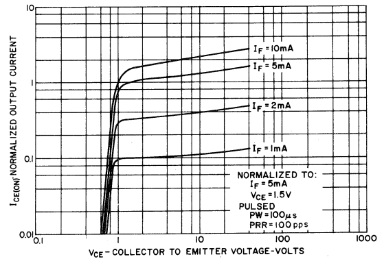
4. OUTPUT CHARACTERISTICS
