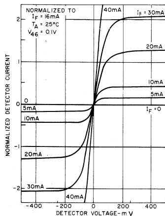
c. HIGH LEVEL V-I PLOT
