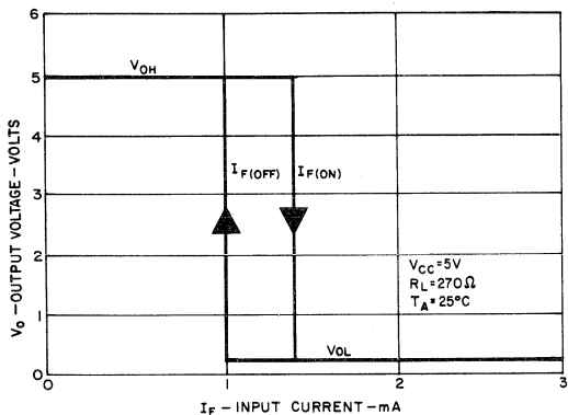
TRANSFER CHARACTERISTICS
