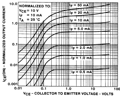
5. OUTPUT CHARACTERISTICS
