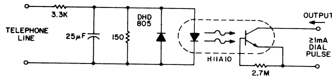
Fig. 113 - Dial pulse indicator.
