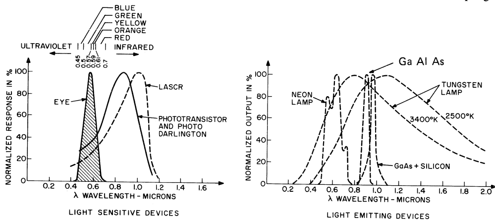
Fig. 15 - Normalized spectral characteristics of light sensitive and light emitting diodes.
