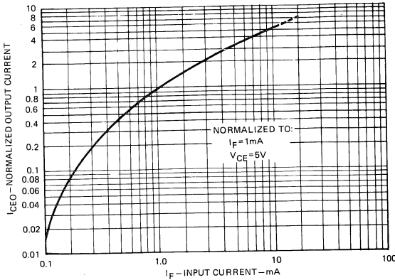
OUTPUT CURRENT VS. INPUT CURRENT
