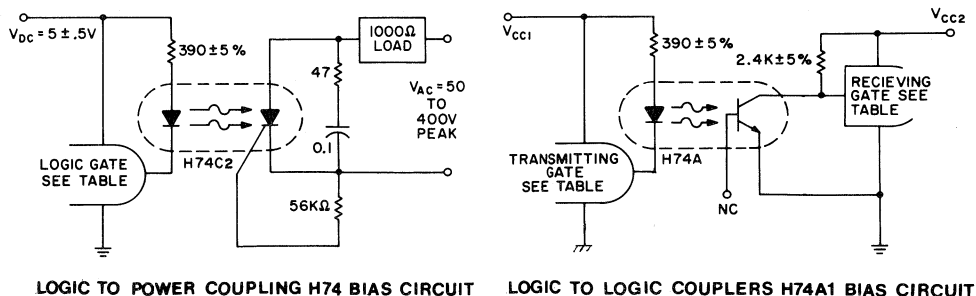
Fig. 103 - H74 series TTL logic coupling.
