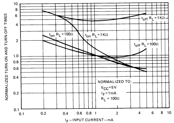
SWITCHING TIMES VS. INPUT CURRENT
