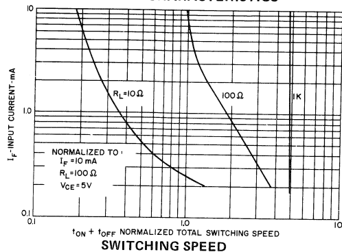
SWITCHING SPEED
