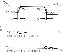
TEST CIRCUIT FOR TRANSIENT IMMUNITY AND TYPICAL WAVEFORMS
