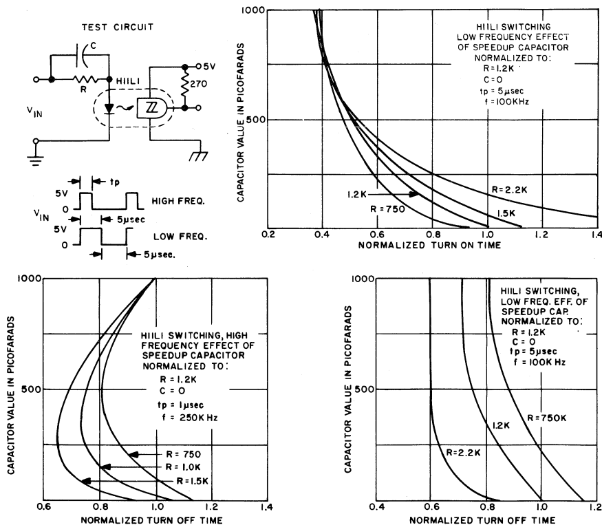
Fig. 55 - H11L switching.
