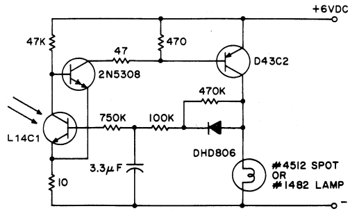
Fig. 82 - Automatic night flashing light.
