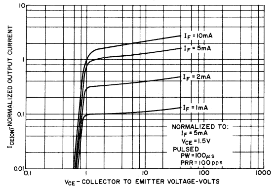
4. OUTPUT CHARACTERISTICS
