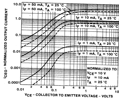
6. OUTPUT CHARACTERISTICS
