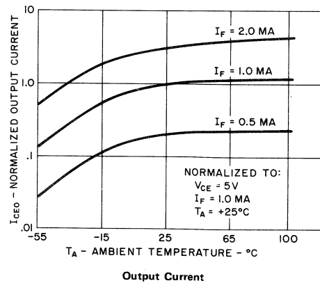
Fig. 44 - Typical temperature effects on photodarlington output.
