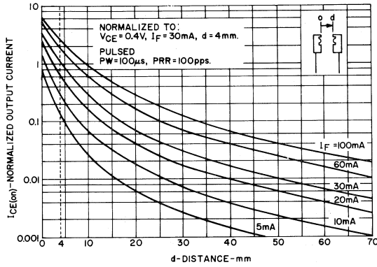
3. OUTPUT CURRENT VS. DISTANCE
