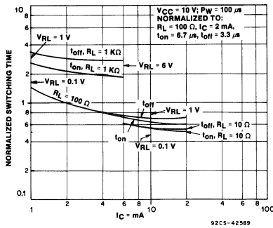
11. SWITCHING SPEED VS. COLLECTOR CURRENT (NOT SATURATED)
