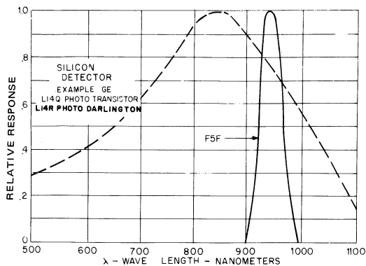
5. SPECTRAL RESPONSE
