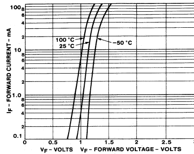
INPUT CHARACTERISTICS
