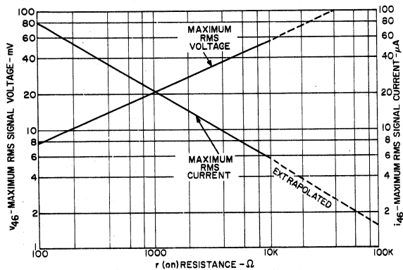
5. REGION OF LINEAR RESISTANCE
