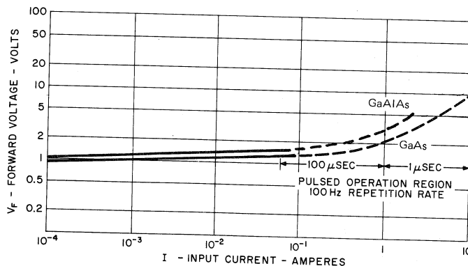
Fig. 32 - Typical optocoupler input characteristics — V_F vs. I_F at 25°C.
