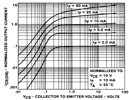
OUTPUT CHARACTERISTICS
