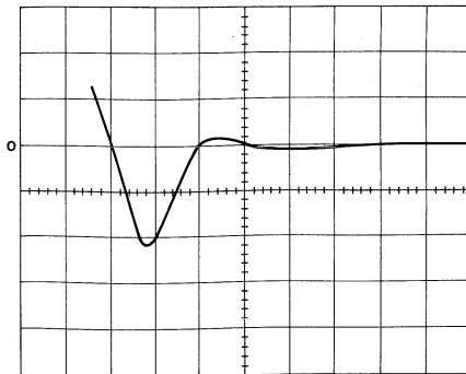
c) TURNOFF WAVEFORM WITH V_{BB} TO INCREASE LOAD VOLTAGE TO 75\text{V} V = 50 \text{ V/DIVISION} t = 50 \text{ ns/DIVISION}
