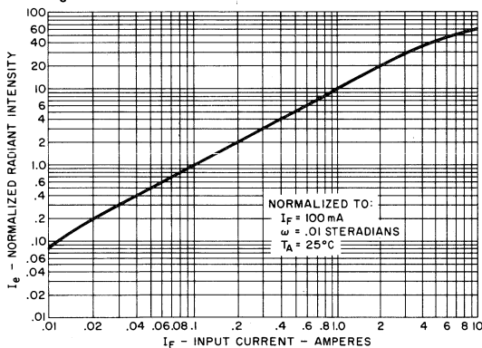
1. RADIANT INTENSITY VS. INPUT CURRENT \Delta I_e/\Delta I
