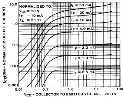
5. OUTPUT CHARACTERISTICS
