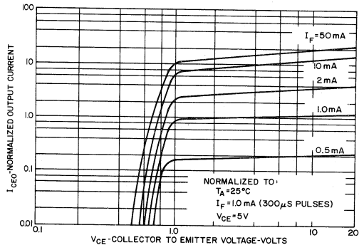
OUTPUT CHARACTERISTICS
