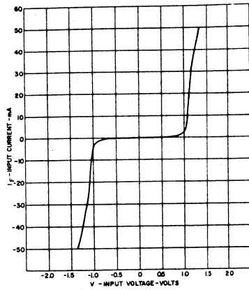
1. INPUT CHARACTERISTICS
